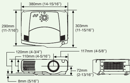
CP-X880/CP-X885 Dimensions (incl.protruding part)
